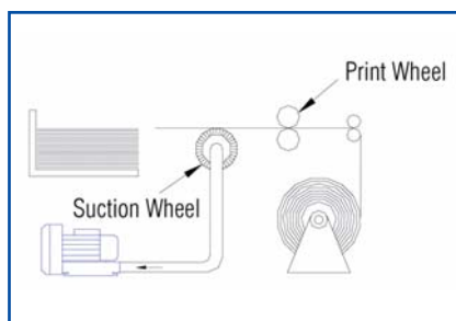
Impresoras Printing Paper Conveyor
