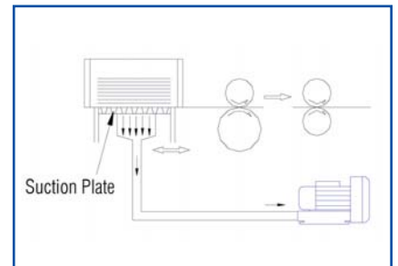
Transporte de papel Paperboard Conveyor
