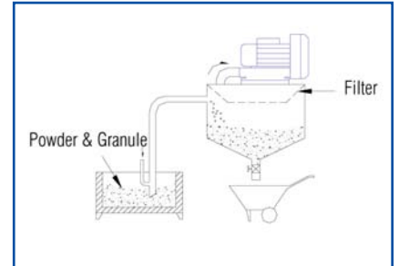
Transporte de grano Powder & Granule Conveyor
