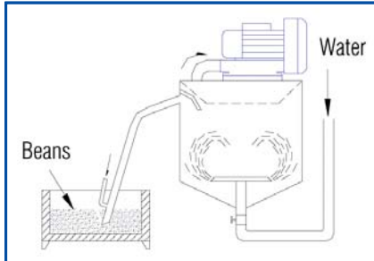
Lavado de legumbres Bean Washing Equipment
